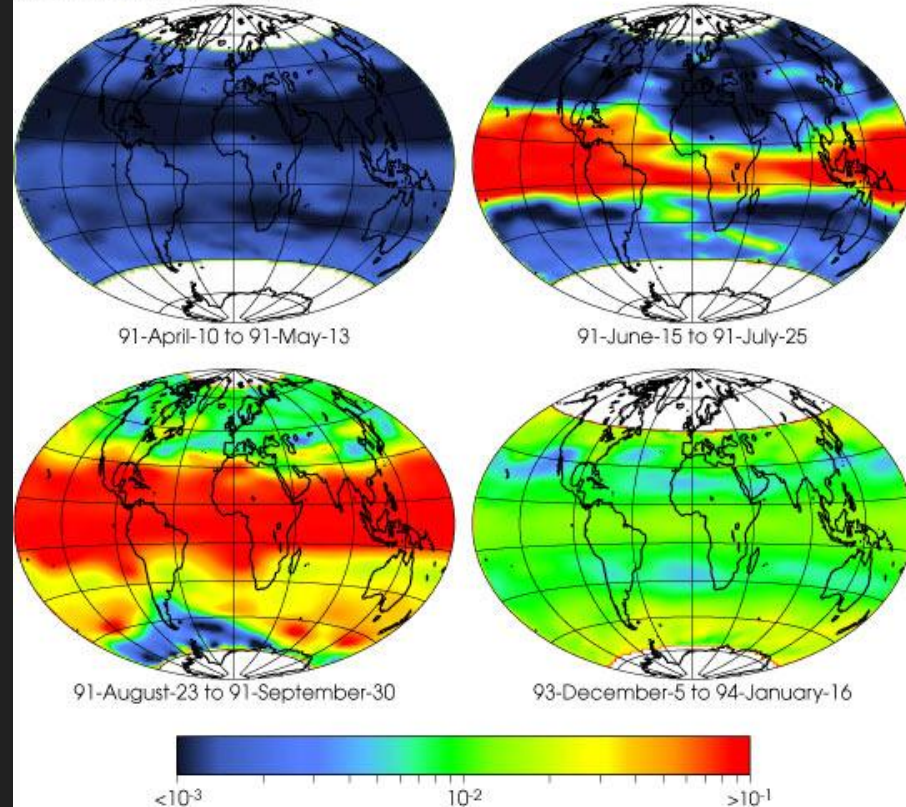
SAGE II 1020 nm Optical Depth
