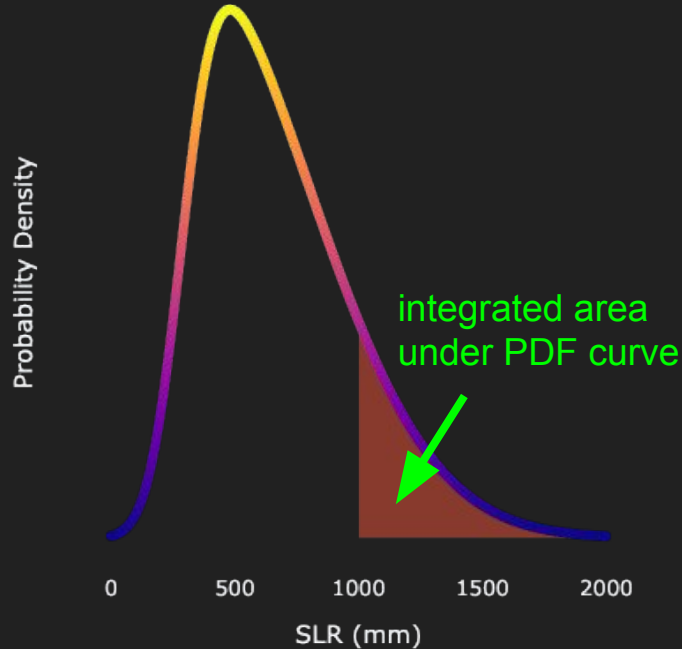
2100 Global SLR Probability Dist.
