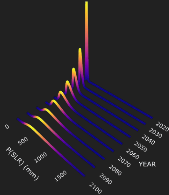
Global SLR Probability Dist. by Year
