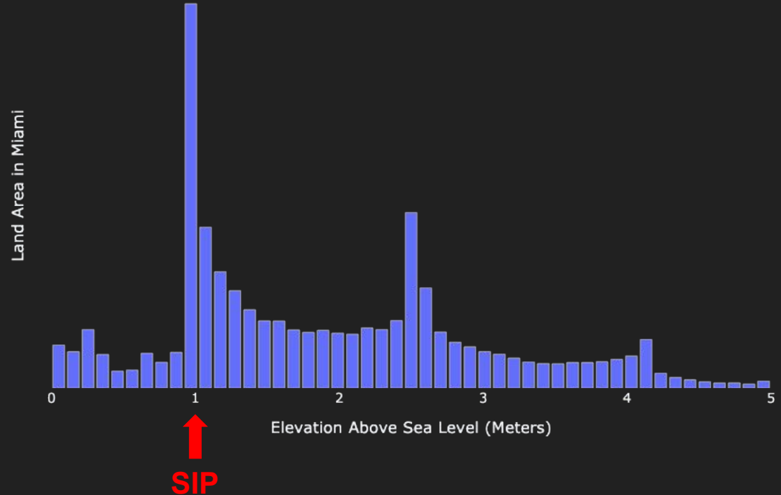
Miami Elevation Distribution
